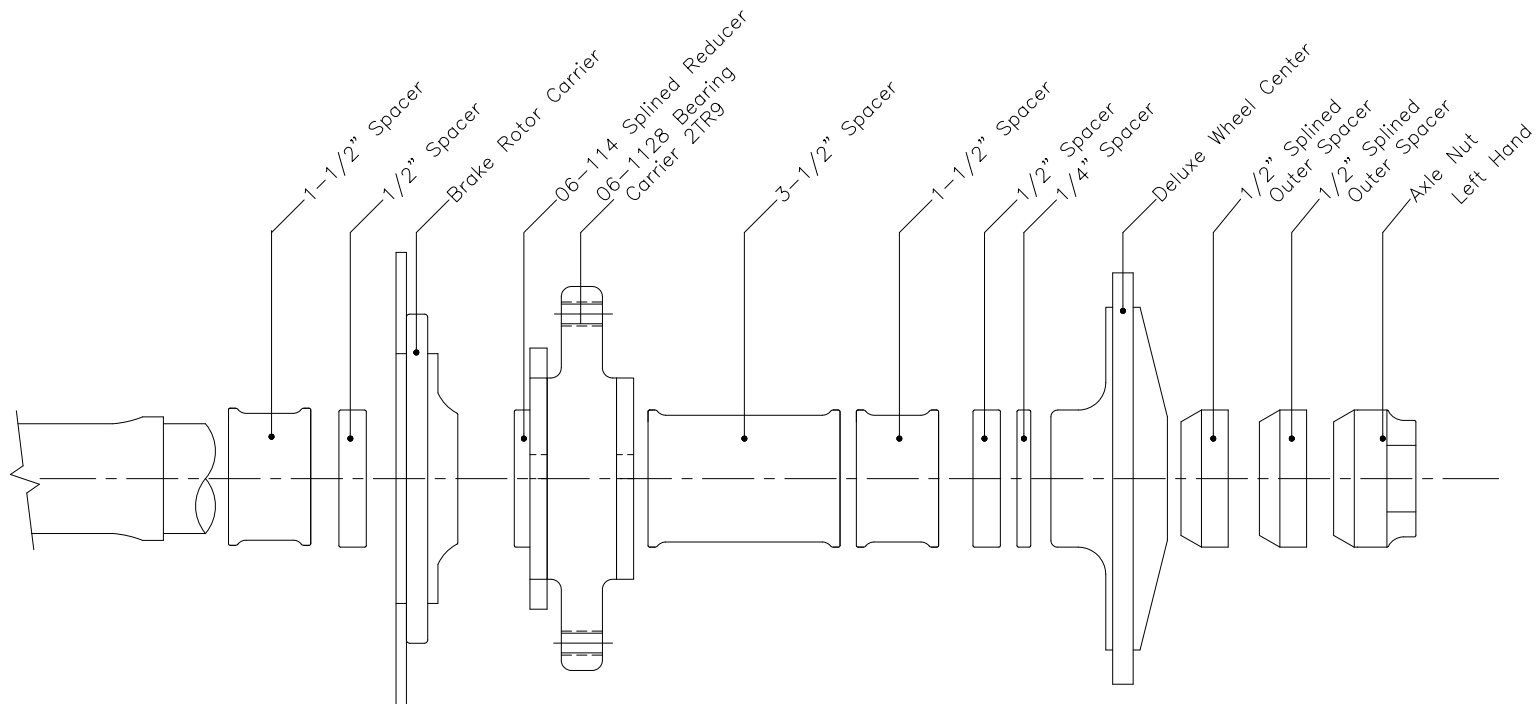
Right Side of 2" Torsion Panhard Bar Axle
