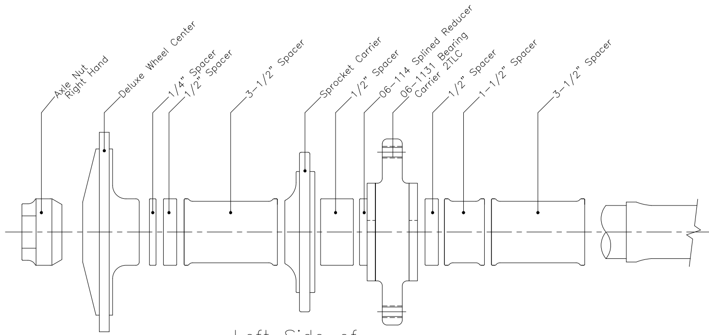
Left Side of 2" Torsion Panhard Bar Axle
