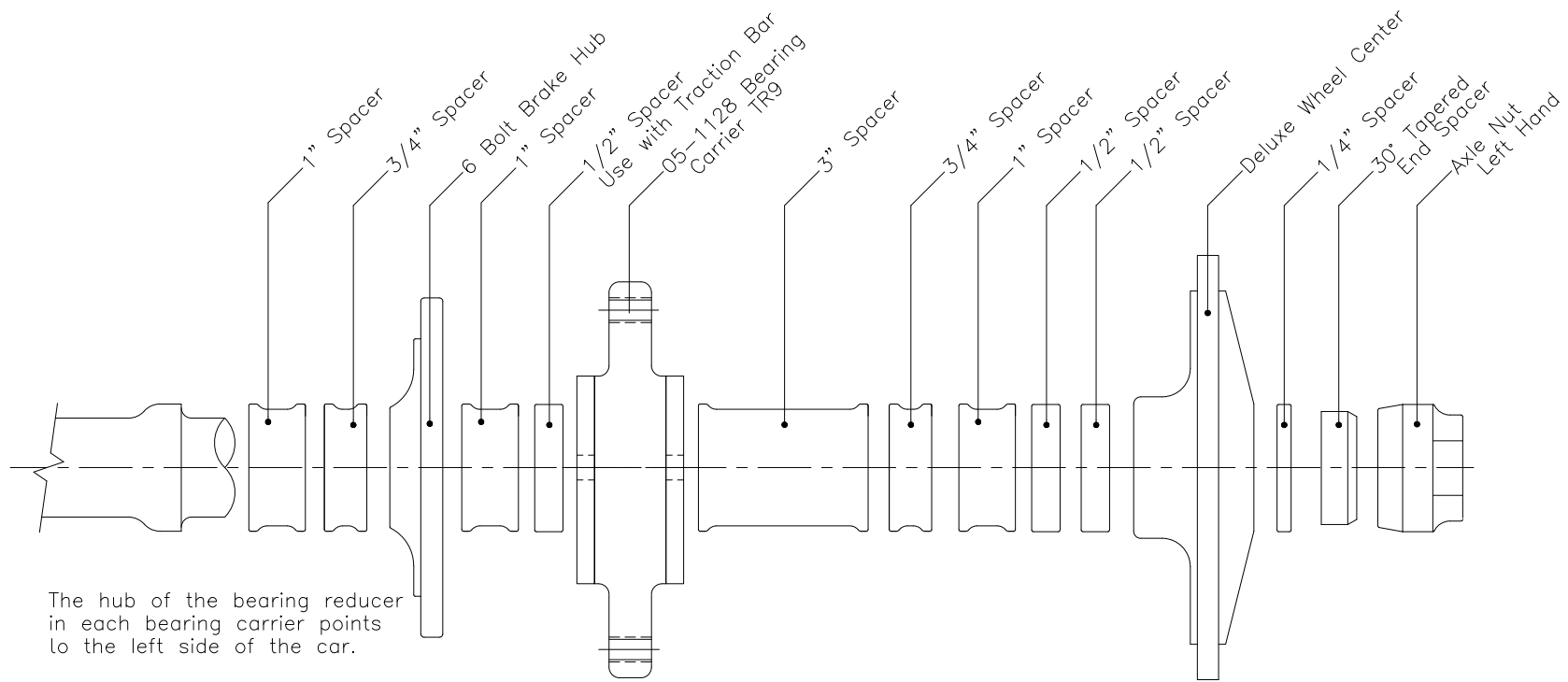
Right Side Torsion 1-3/4" Axle Panhard Bar
